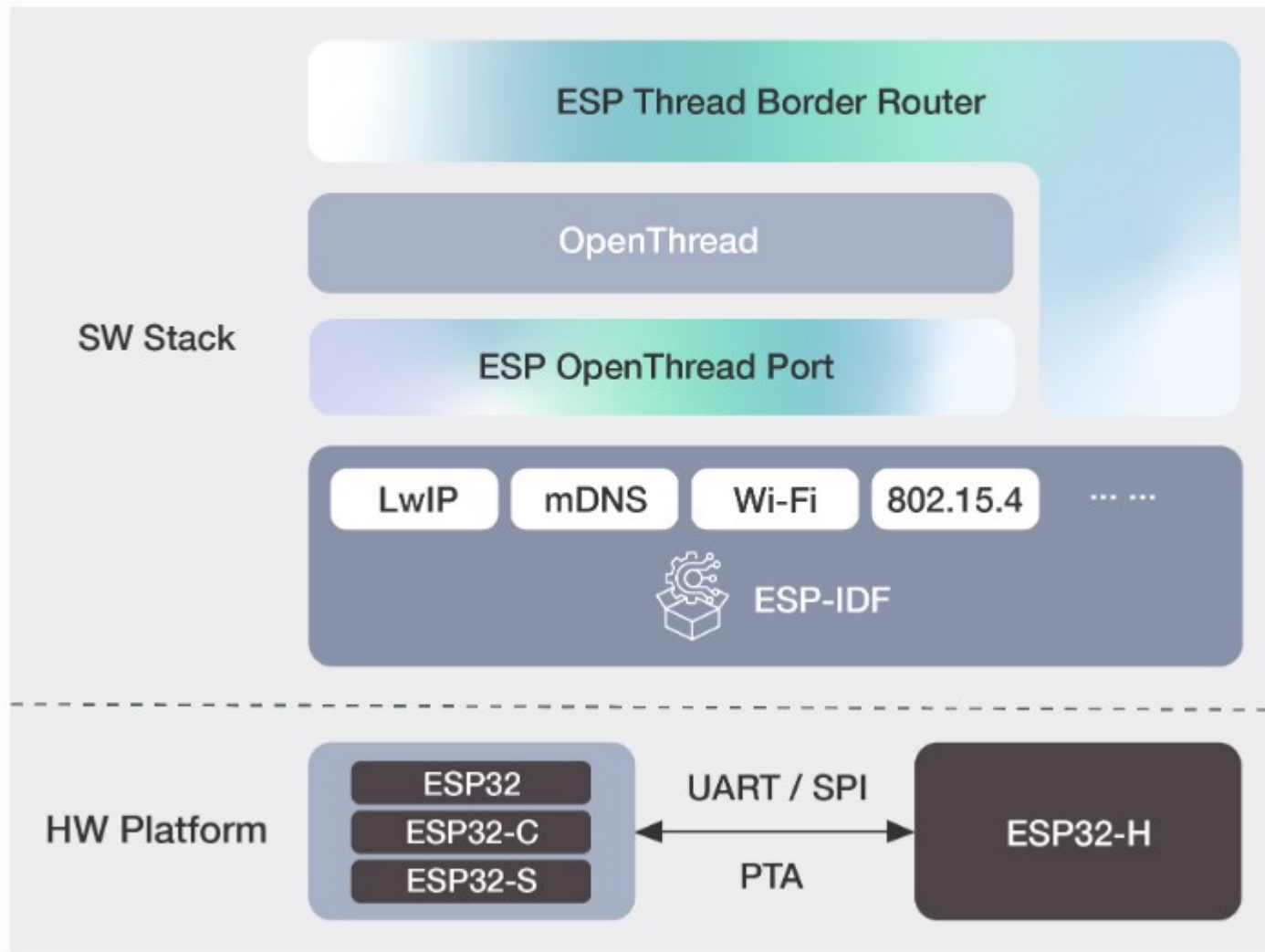
ESP-Thread-Border-Router Software Components
